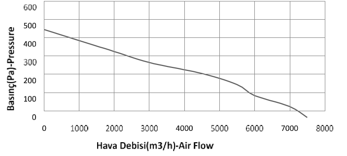
GDKF 710 AX
