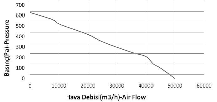
GRRF 1000 AX
