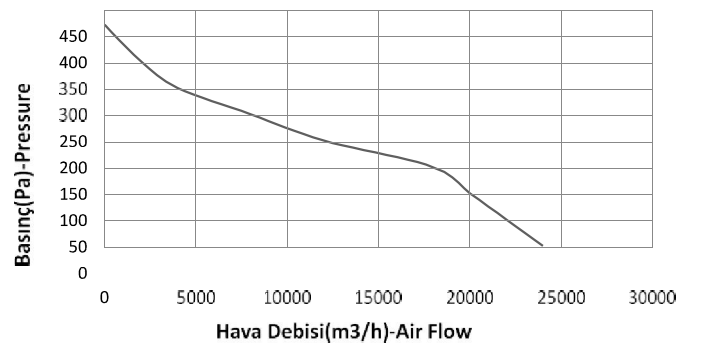
GRRF 800 AX
