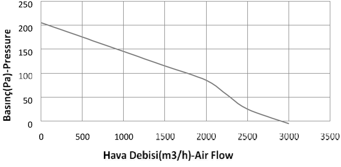
GRRF 500 AX
