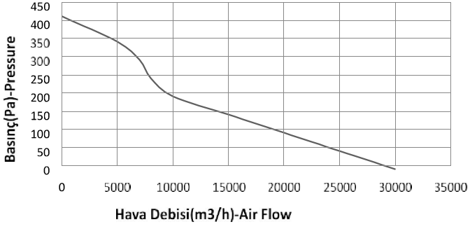
GRRF 900 AX
