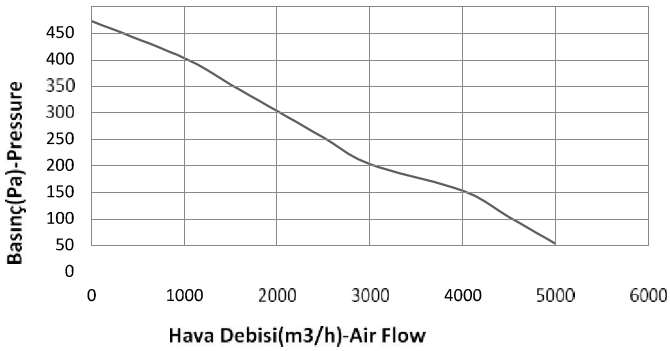
GRRF 800 AX
