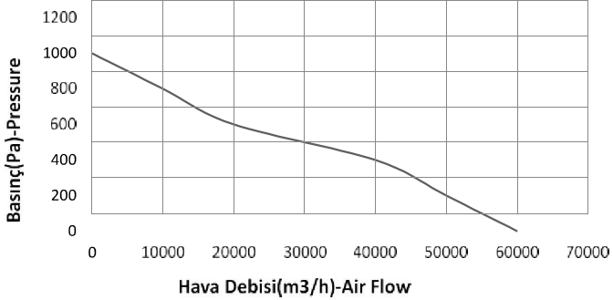
GRRF 1120 AX
