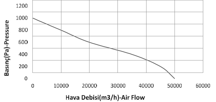
GRRF 1120 AX
