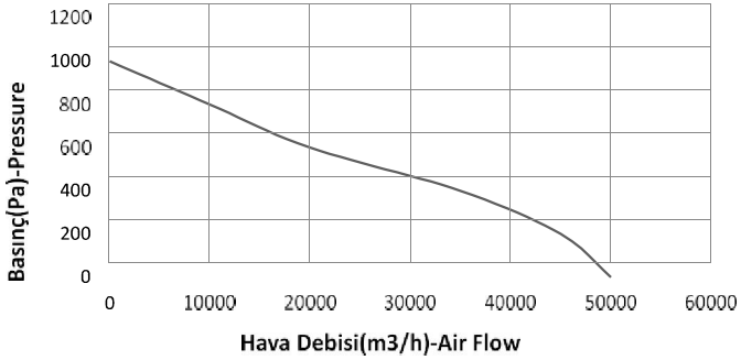
GRRF 1000 AX
