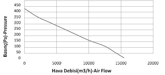
GRRF 800 AX
