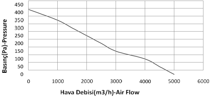
GRRF 630 AX
