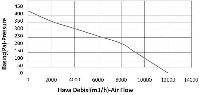
GRRF 800 AX
